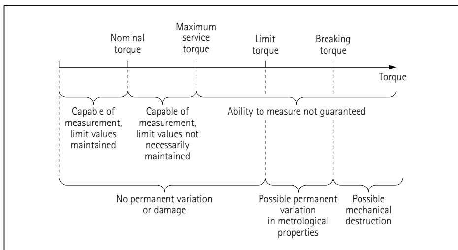
図6 限界負荷 (Load limits)
