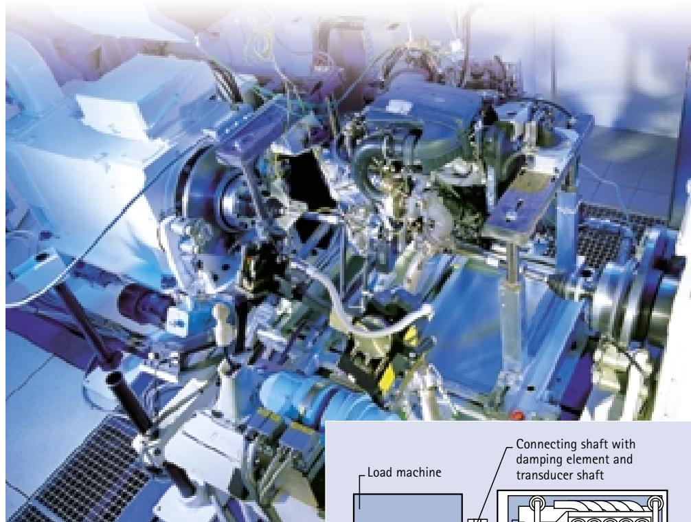
Fig. 1a: Power test stand with integrated torque flanges
