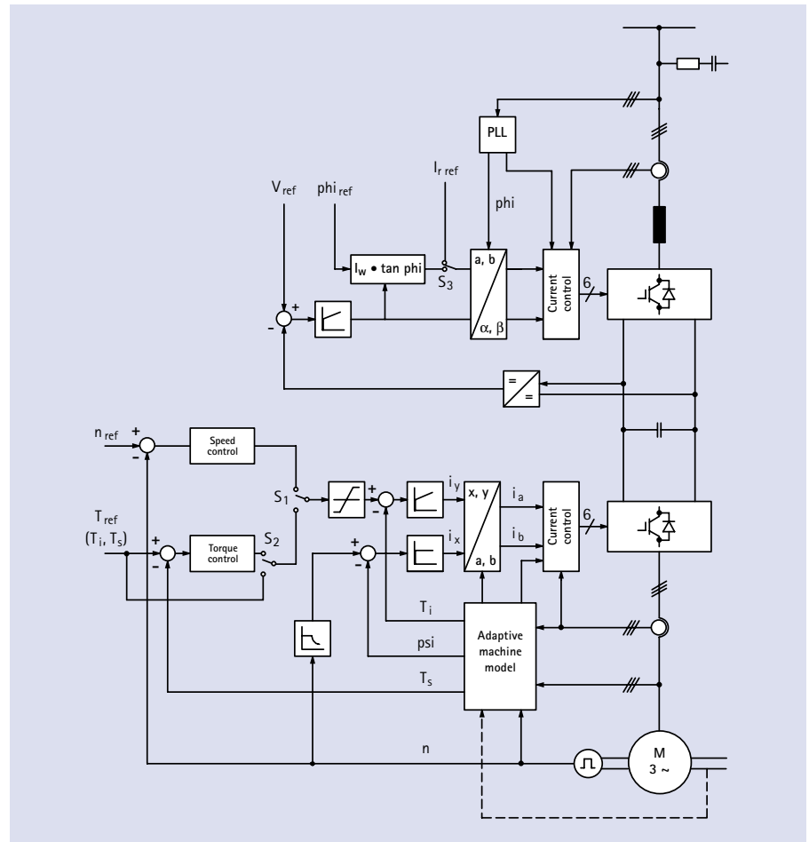
Fig. 4: Basic structure of machine control with integrated torque computer and returned measured moment
