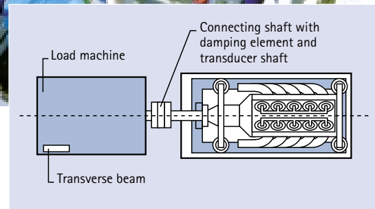
Fig. 2a: Basic structure of a typical engine test stand
