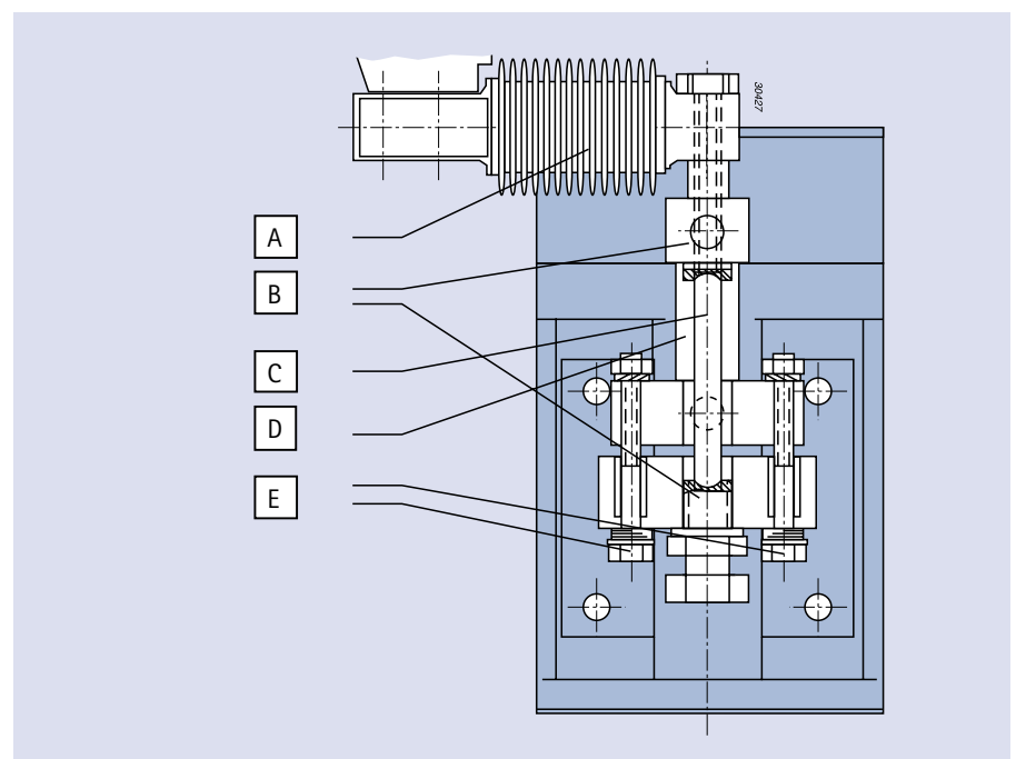
Fig. 2: Mechanical construction with measurement option in the direction of compression and tension, as well as compensation for a certain sideways displacement
