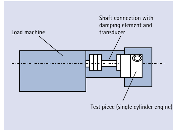
Fig. 9: Single cylinder test stand layout using the T10F-SVL torque flange
