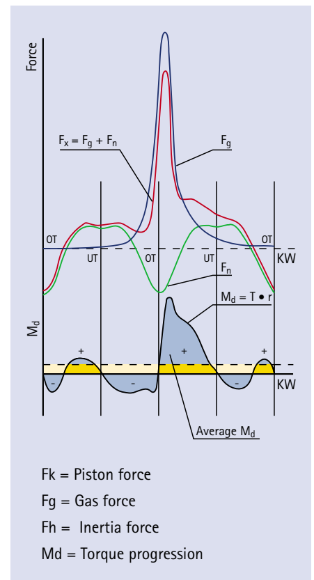
Fig. 6: The engine transmission forces of a combustion engine and the resultant torque progression
