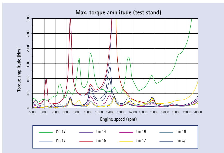
Fig. 13: Moment amplitudes in some sections of the drive train. The transducer shaft is arranged in position 16
