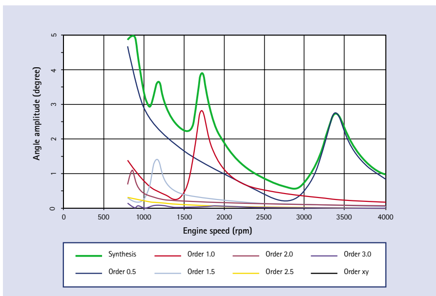
Fig. 11: Angle amplitudes of the individual engine orders in the measurement system range
