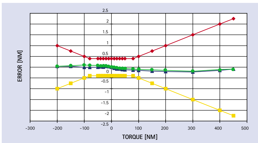
Fig. 3: This shows the typical calibration curve with the hysteresis characteristic of an APA with hydrostatic bearings
