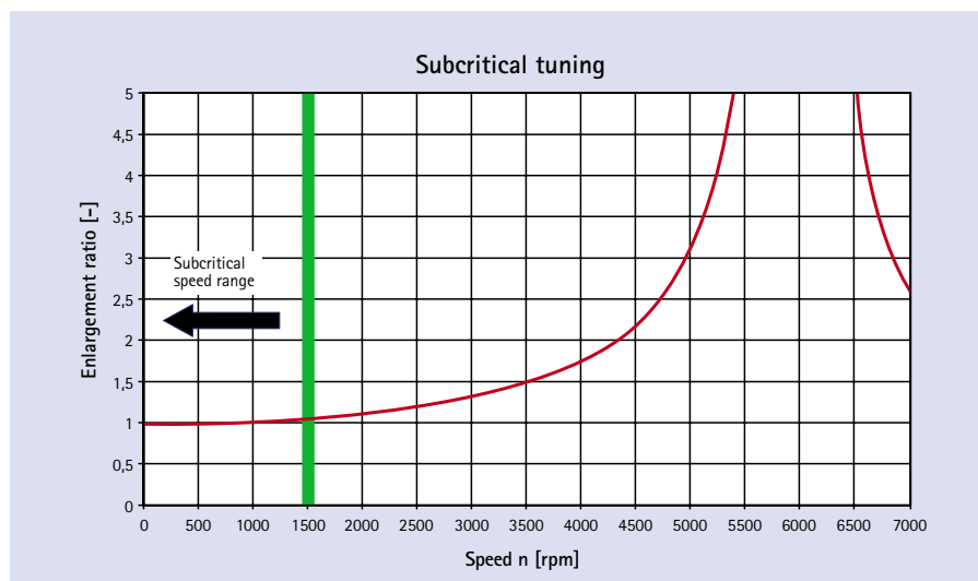
Fig. 8: Operating range for the subcritical design
