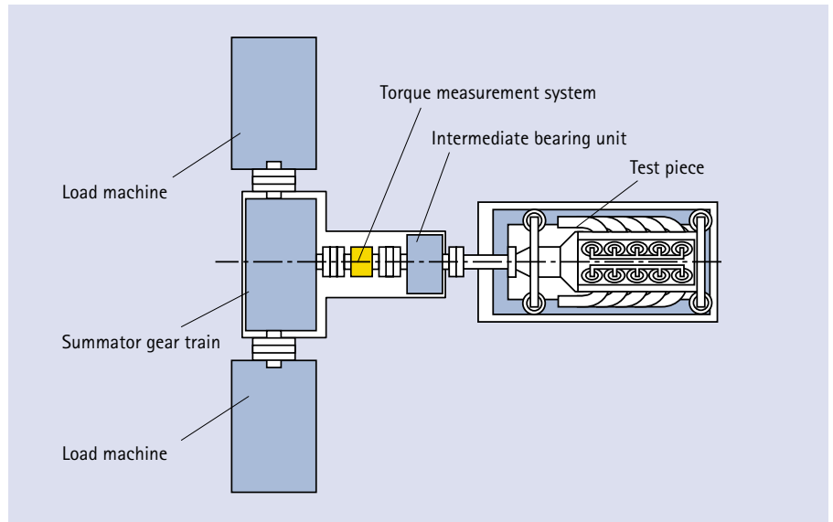
Fig. 12: Typical highly-dynamic racing test stand
