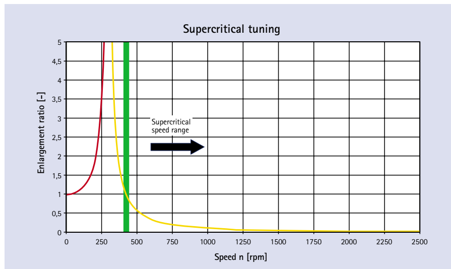
Fig. 7: Operating range for the supercritical design
