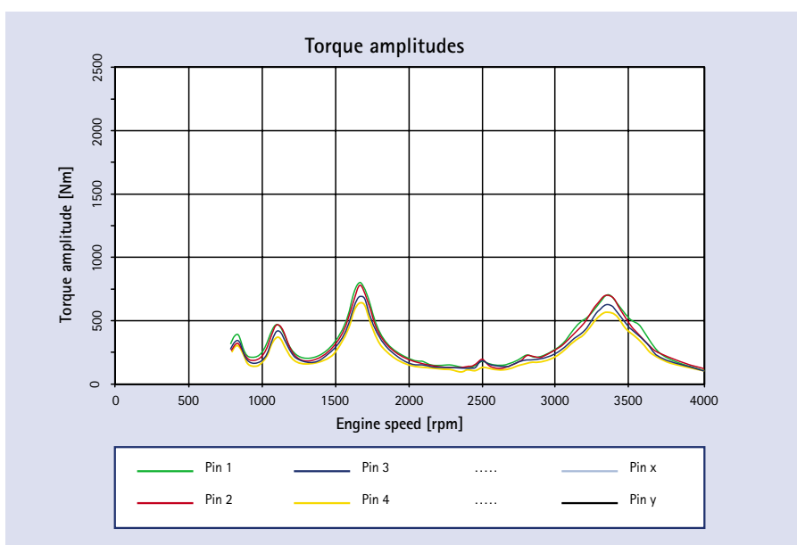
Fig. 10: Torque amplitudes in the individual sections of the drive train. The measurement system is in the range identified by pin 3
