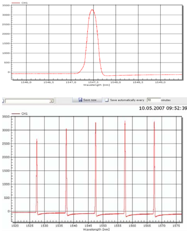
Fig. 20: Wavelength spectrum
