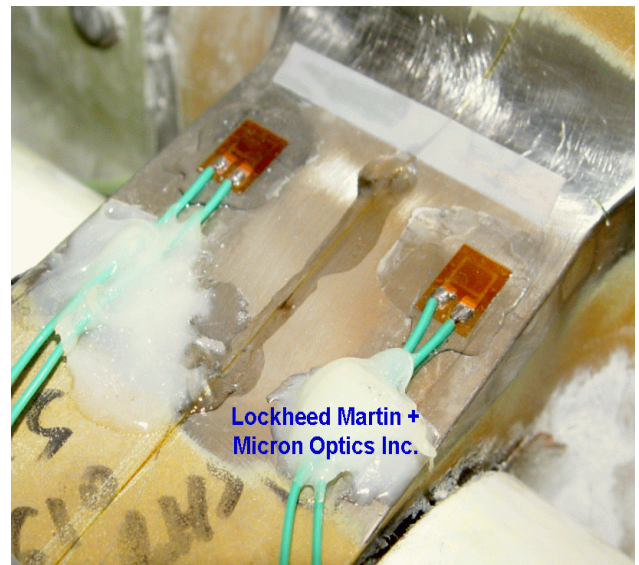
Fig. 14: Application of two strain gages and one FBG sensor
