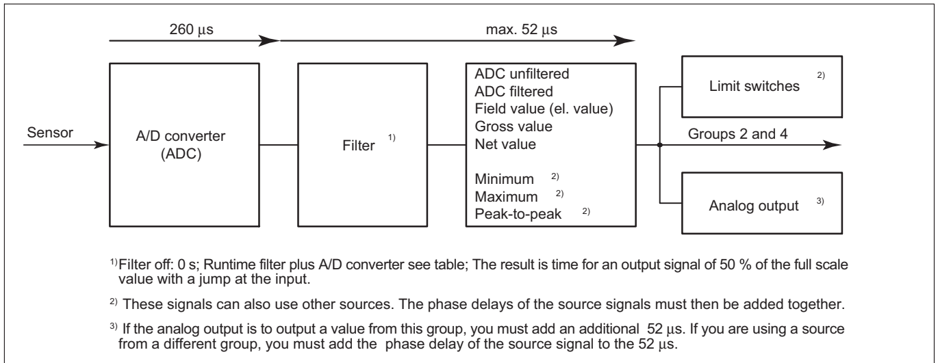
Fig. 1: Minimum phase delays for group 1: 52 ms plus A/D converter conversion time plus filter runtime
