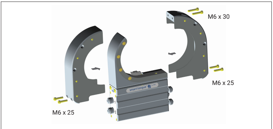
Fig. 8.10 Fitting the two halves of the protection against contact
