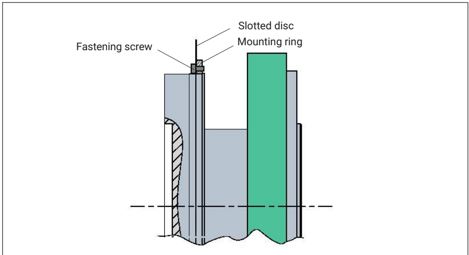
Fig. 8.1 Installing the slotted disc
