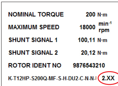
Fig. 23.3 Stator sticker: rotor hardware revision version
