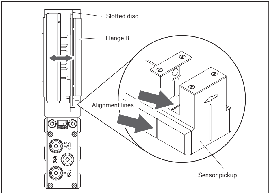
Fig. 8.21 Position of the slotted disc in the speed sensor
