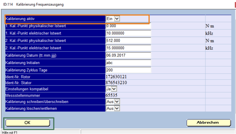
Fig. 14.3 Calibration information for TEDS, frequency output
