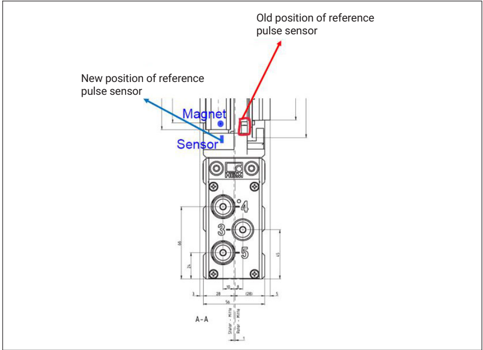
Fig. 23.5 New position of the reference pulse sensor, valid from stator hardware version 3.xx
