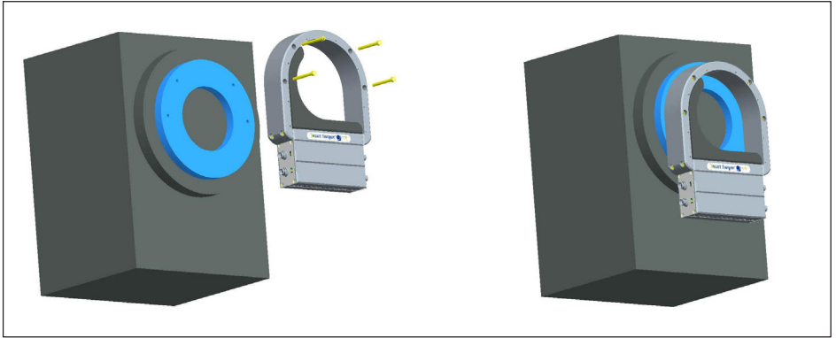
Fig. 8.20 Face-mounting on the customer side engine shielding
