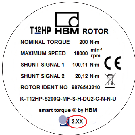
Fig. 23.4 Rotor sticker: rotor hardware revision version
