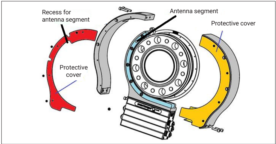
Fig. 8.8 Protective cover T12HP
