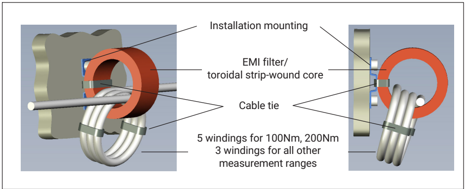
Fig. 10.1 EMI filter/toroidal strip-wound core installation example
