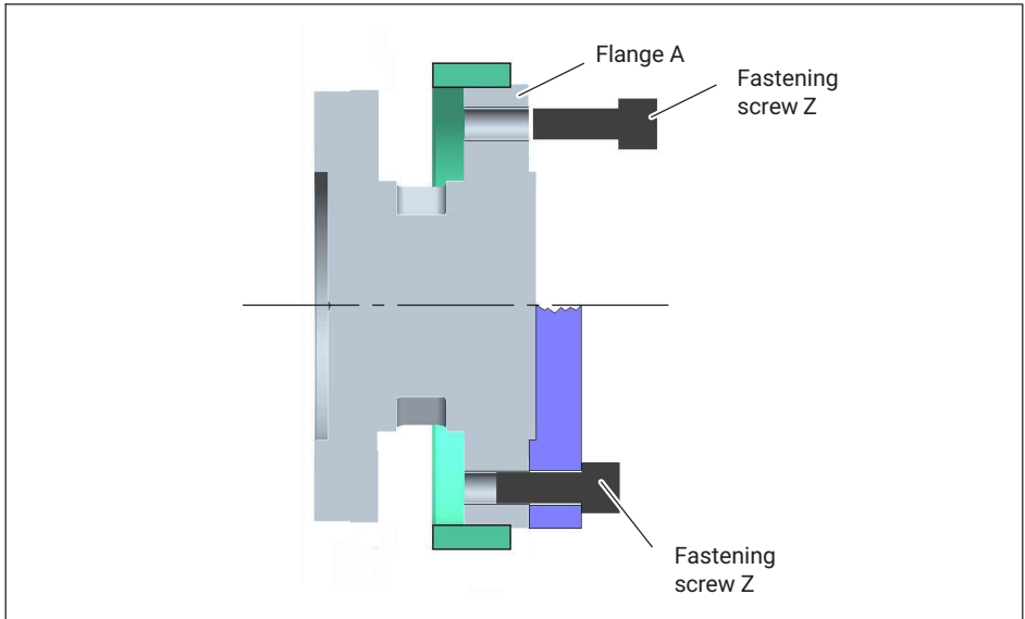
Fig. 8.3 Screw connections, flange A
