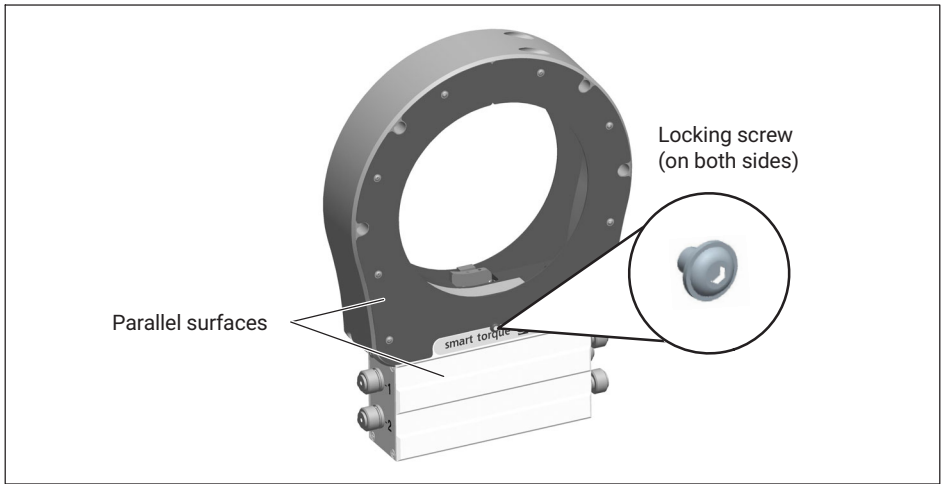
Fig. 8.11 Check for parallelism
