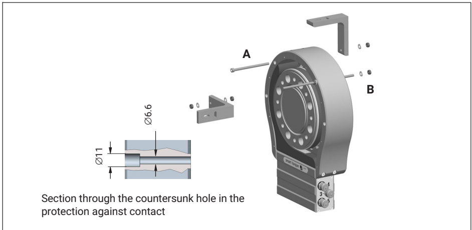
Fig. 8.14 Supporting the stator with protection against contact
