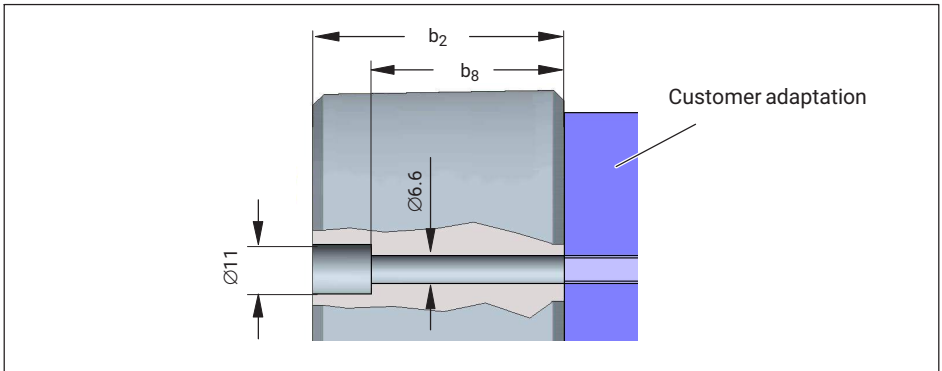
Fig. 8.19 Mounting holes in the protection against contact
