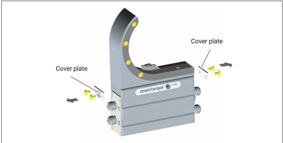
Fig. 8.4 Cover plates on the stator housing
