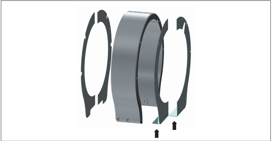
Fig. 8.9 Angled cover plates (5 kN · m and 10 kN · m measurement ranges)
