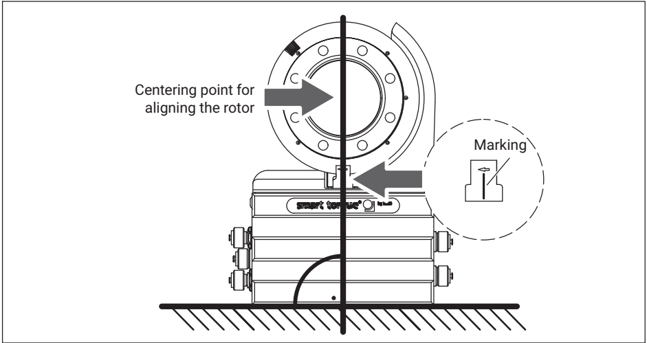
Fig. 8.22 Alignment markings on rotor and stator
