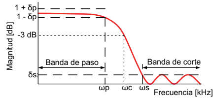
Figura 18: Filtro Bessel IIR digital
