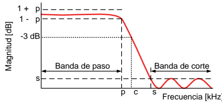
Figura 20: Filtro Butterworth IIR digital
