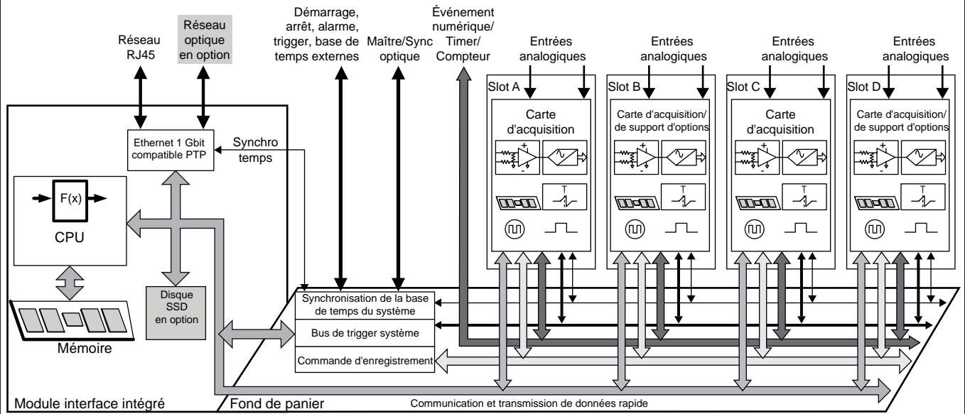
Figure 7 : Synoptique
