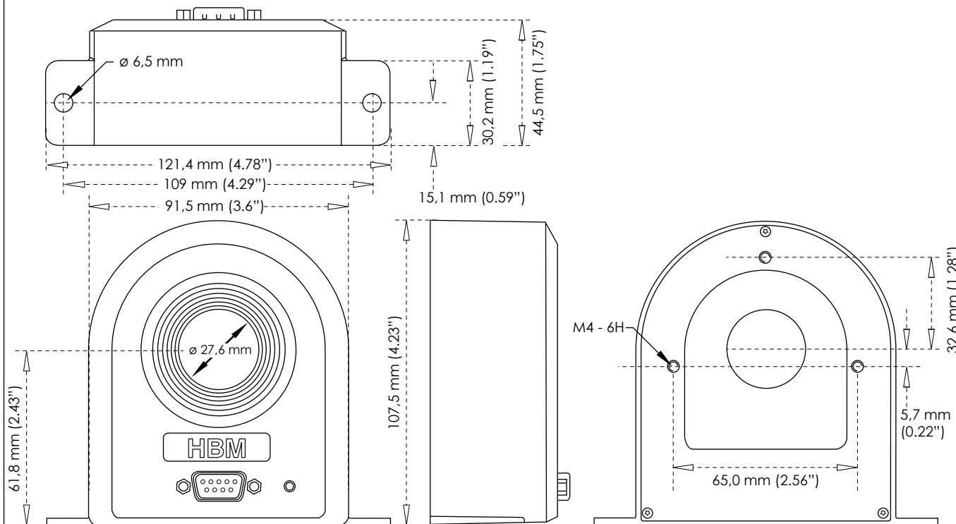
Figure 1.5 : Dimensions CTS50/200ID/400ID/600ID
