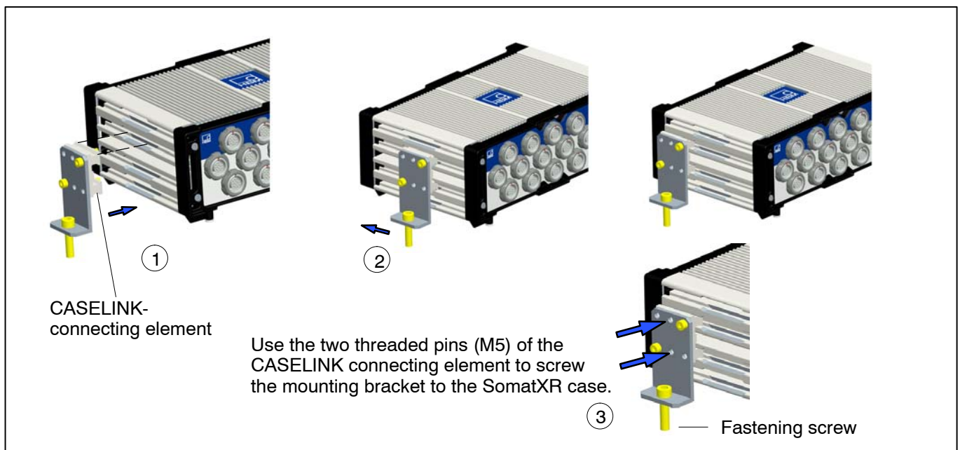
Fig. 2: CASEMOUNT mounting
