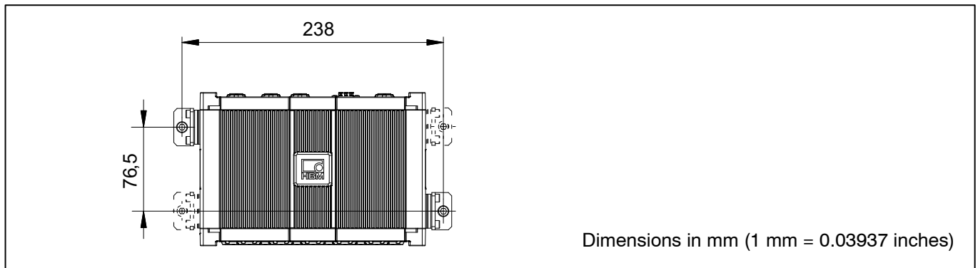
Fig. 1: CASEMOUNT mounting dimensions
