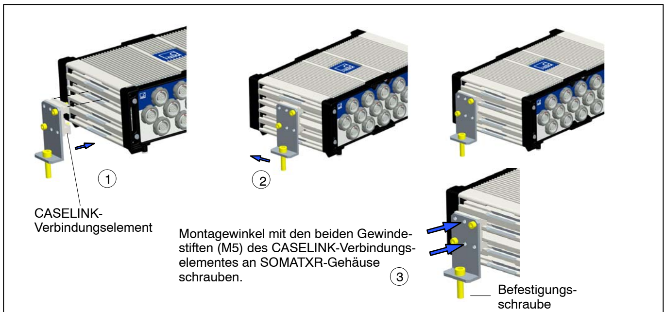
Abb. 2: Montage CASEMOUNT
