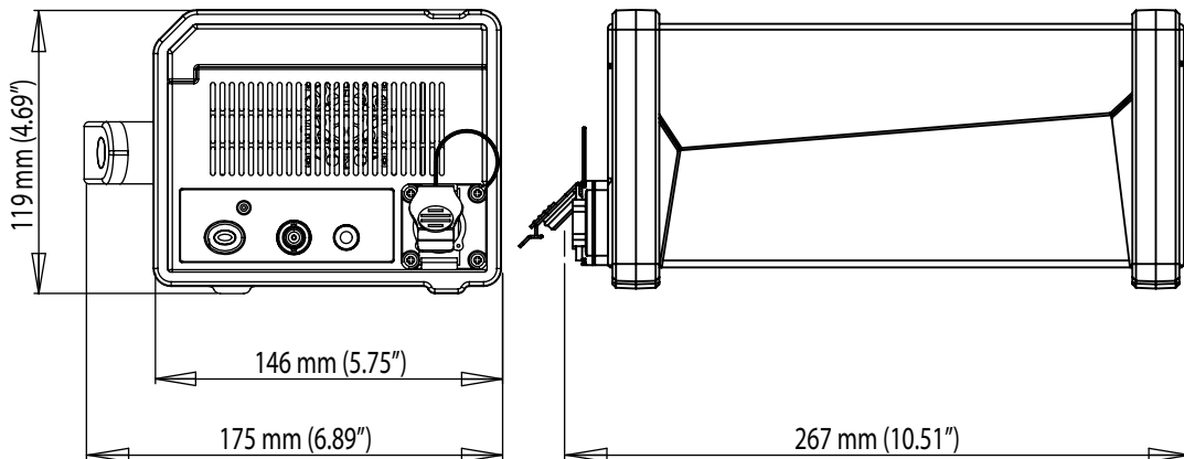
Figure 1.8: Dimensions GN112 and GN113 transmitter
