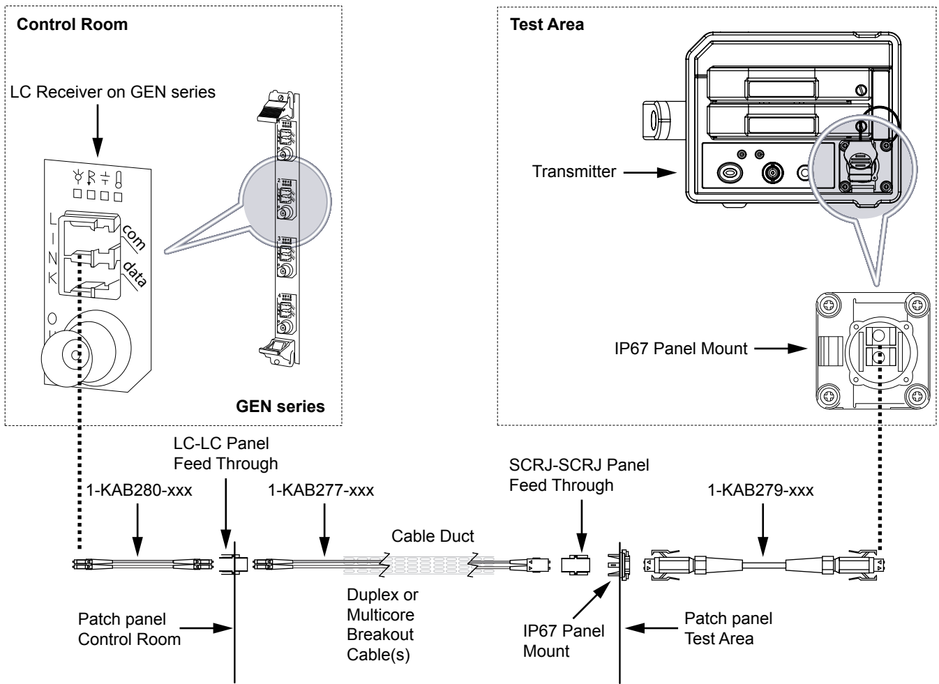
Figure 1.13: Application area of a fiber optic duplex cable (Example 2)
