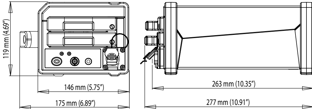
Figure 1.7: Dimensions GN110 and GN111 transmitter
