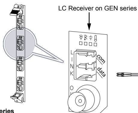
Figure 1.11: Application area of a fiber optic duplex cable (Example 1)
