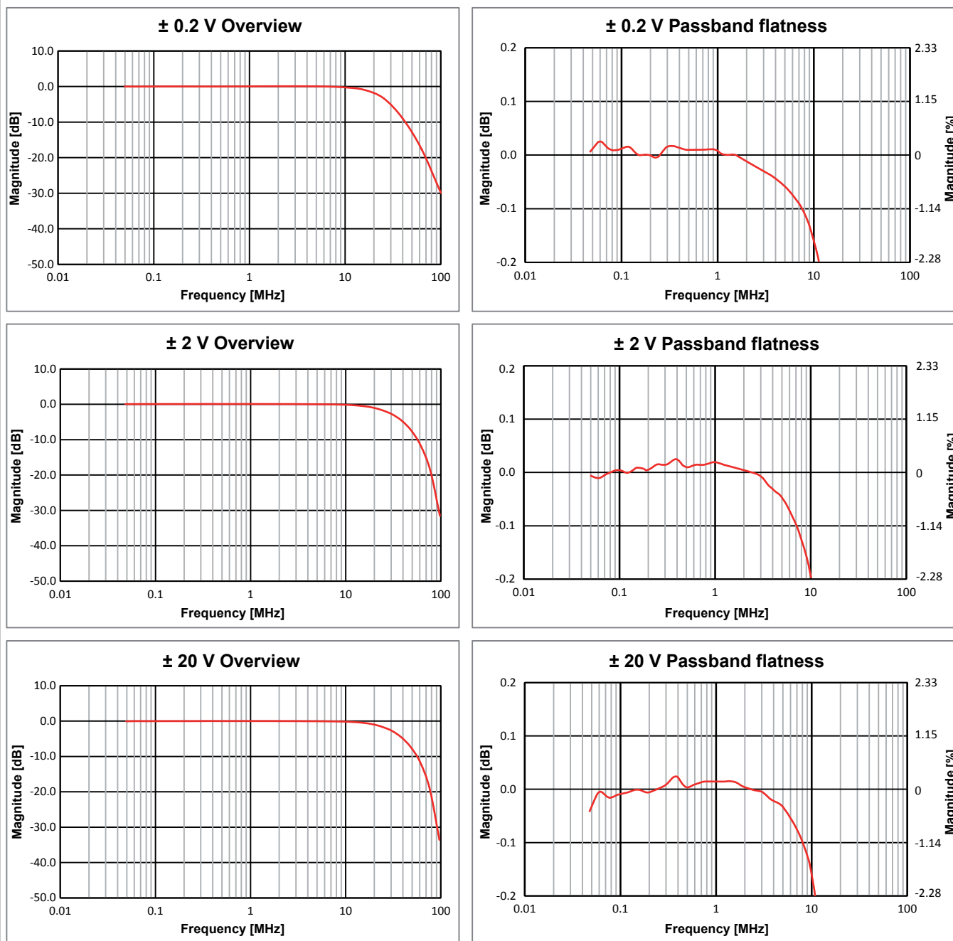
Figure 1.4: Representative Wideband examples
