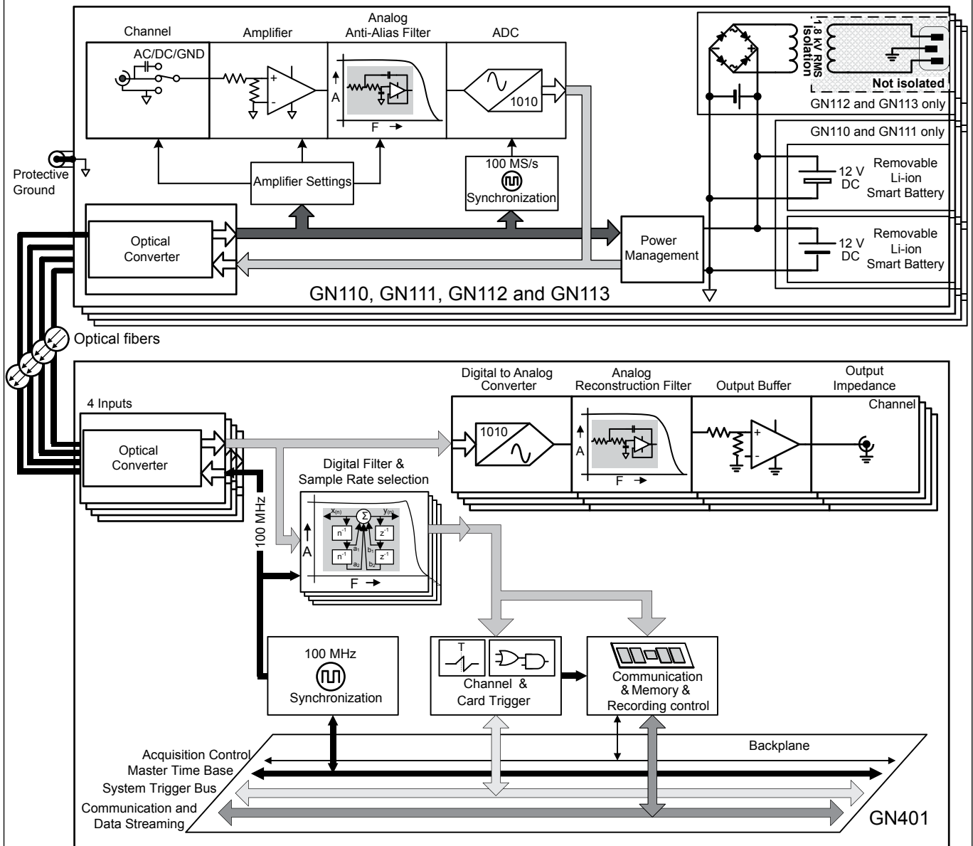
Figure 1.1: Block Diagram GN401 with GN110, GN111, GN112 or GN113
