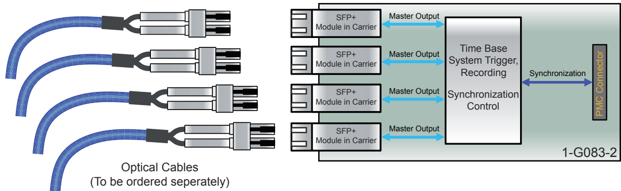
Figure 1.19: Block diagram Master output card (G081 required)
