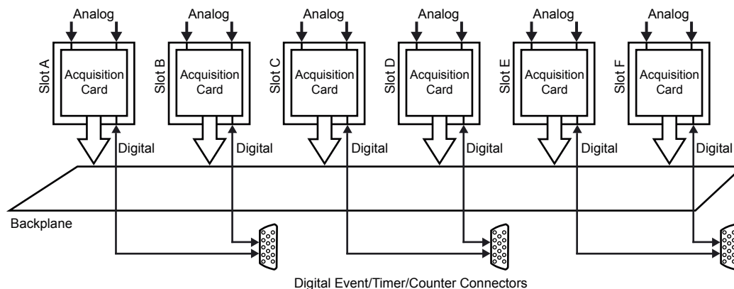
Figure 1.8: Digital Event/Timer/Counter block diagram
