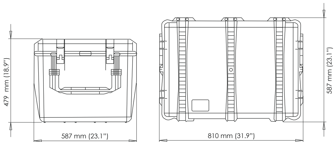
Figure 1.32: Reusable hardcover shipping case with wheels and transport handle
