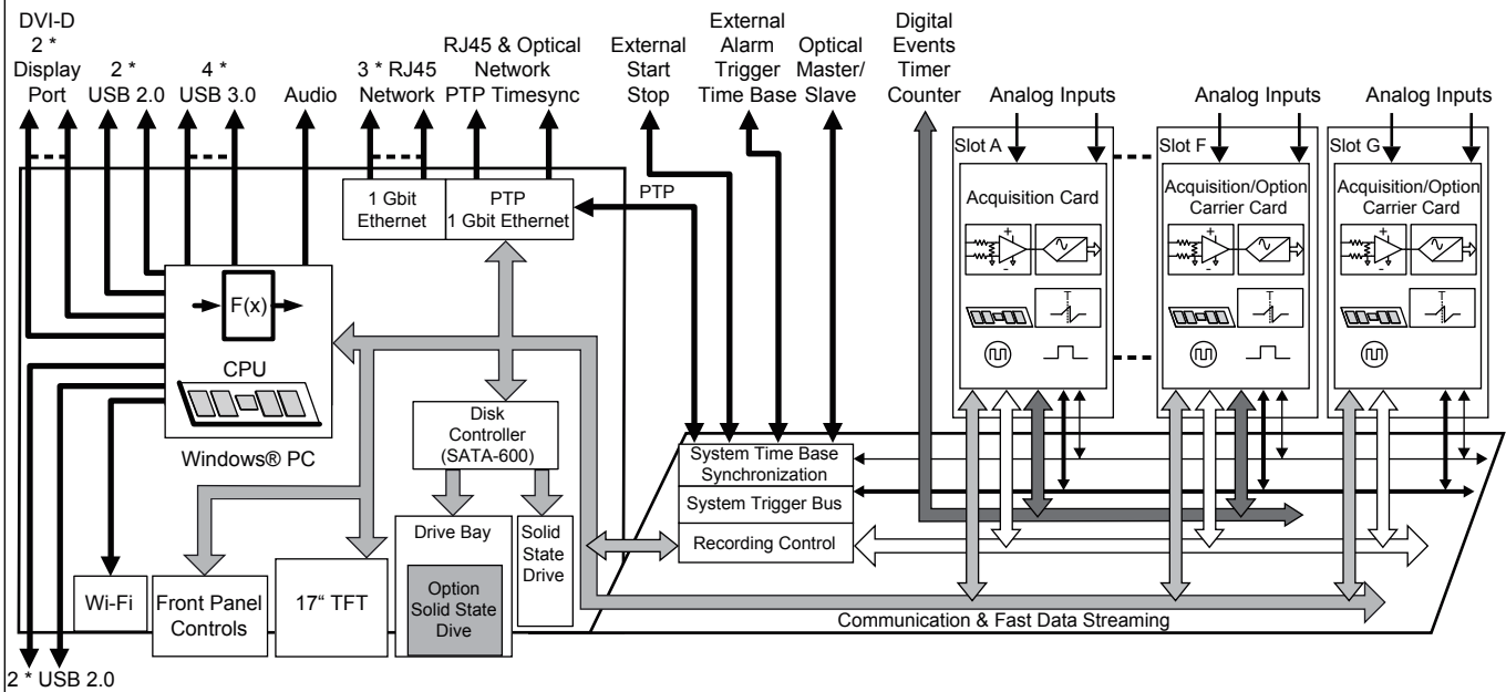
Figure 1.1: Block diagram
