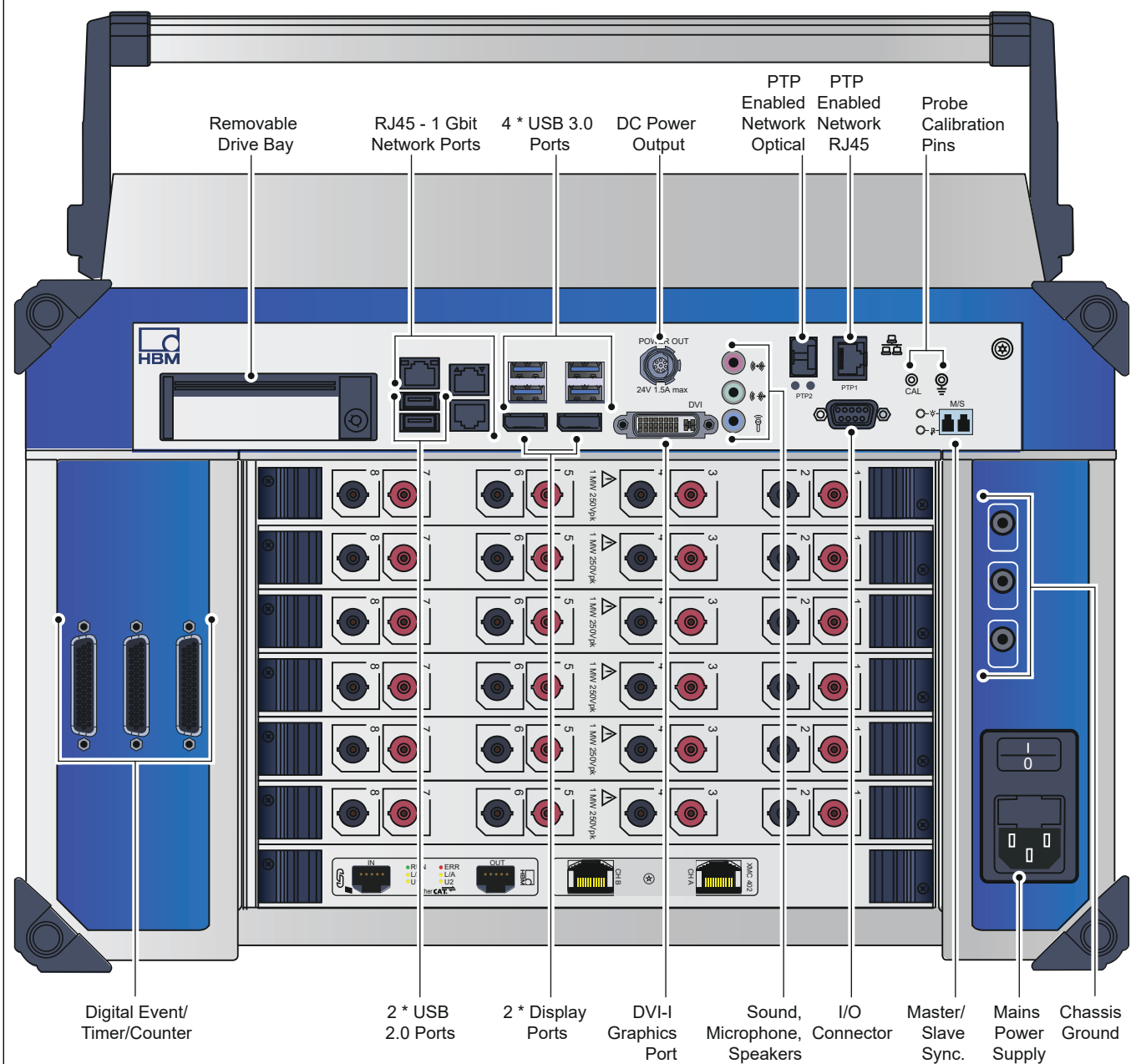
Figure 1.2: Connection overview
