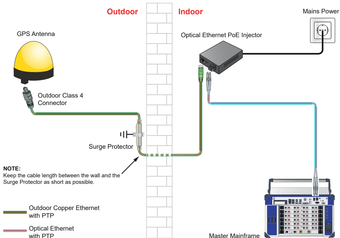
Figure 1.28: Block diagram GPS time synchronization
