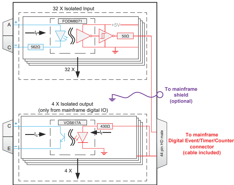
Figure 1.26: Block diagram and image
