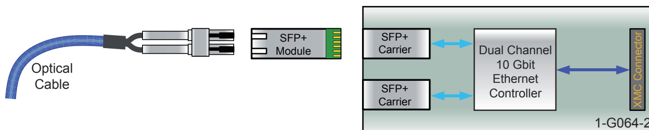
Figure 1.20: Block diagram 10Gbit Ethernet card, optical (G081 required)
