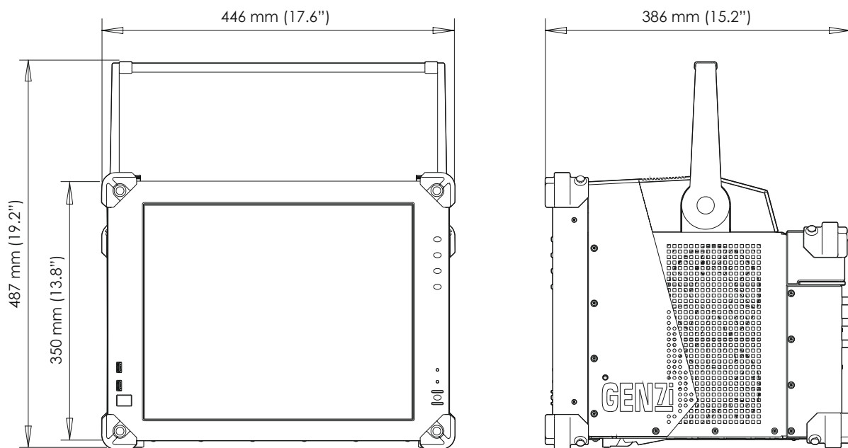
Figure 1.13: GEN7i Dimensions
