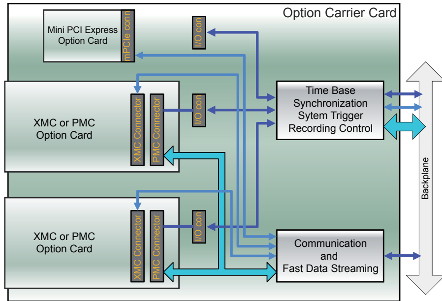
Figure 1.18: Block diagram option carrier card
