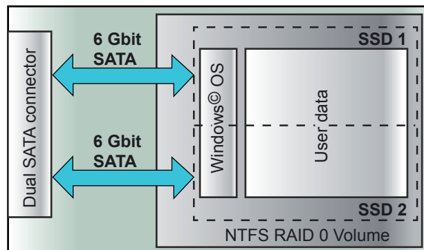
Figure 1.15: Block diagram removable system Solid State Drive
