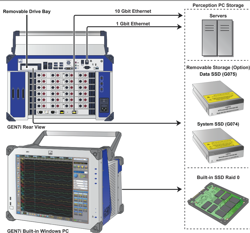
Figure 1.3: Data storage overview
