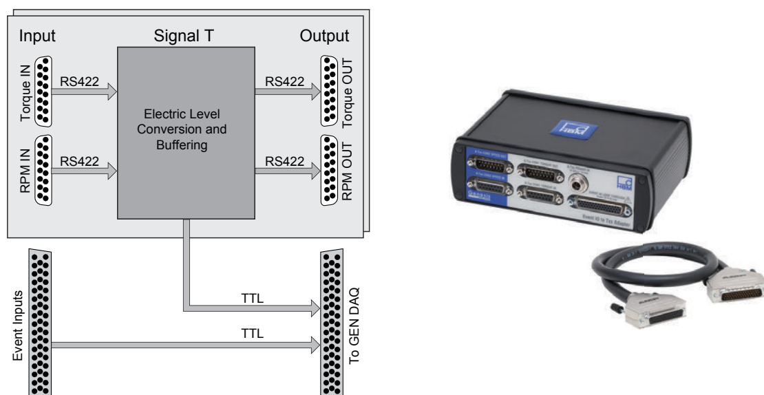
Figure 1.25: Block diagram and image
