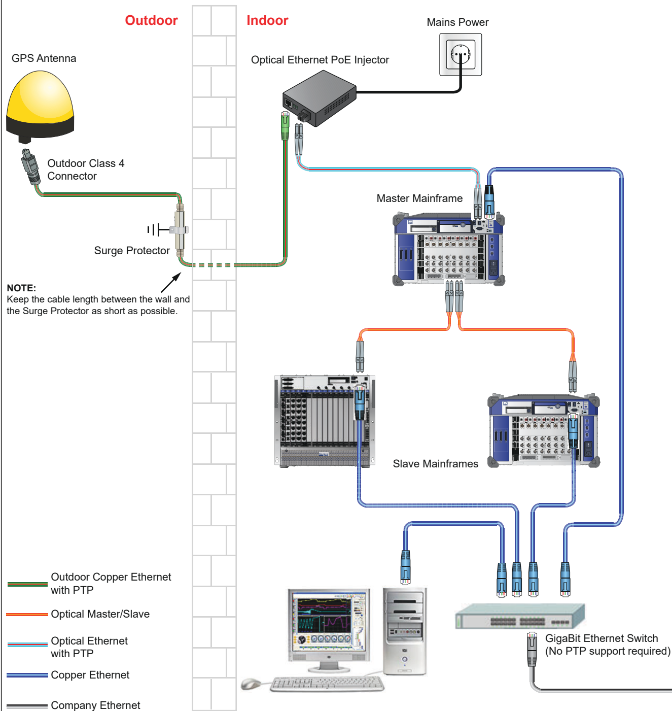
Figure 1.29: GPS setup for tethered mainframe with Master/Slave connected slaves
