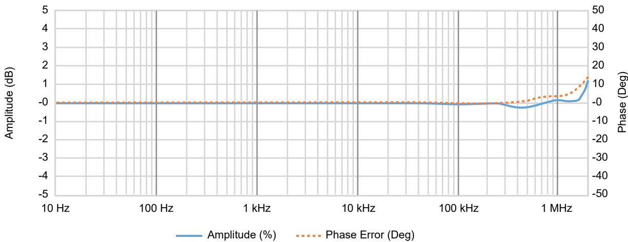
Figure 3: Frequency characteristics
