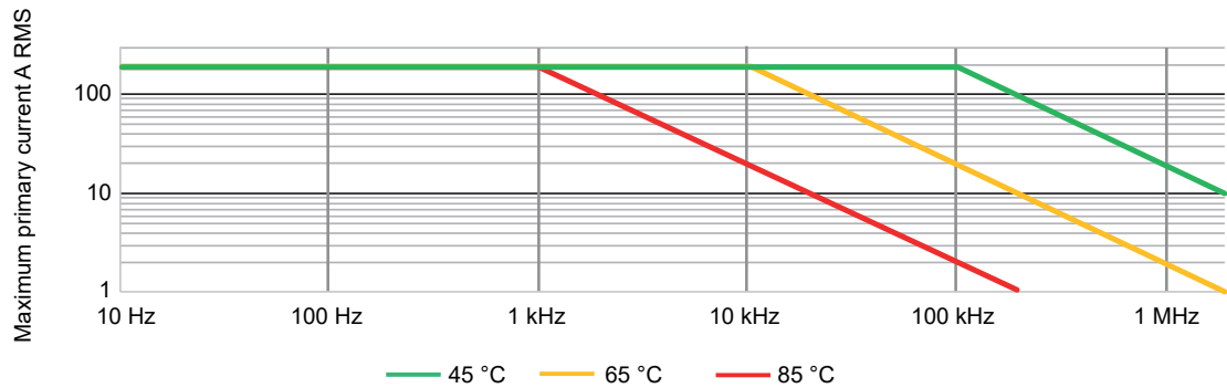
Figure 2: Frequency and ambient temperature derating
