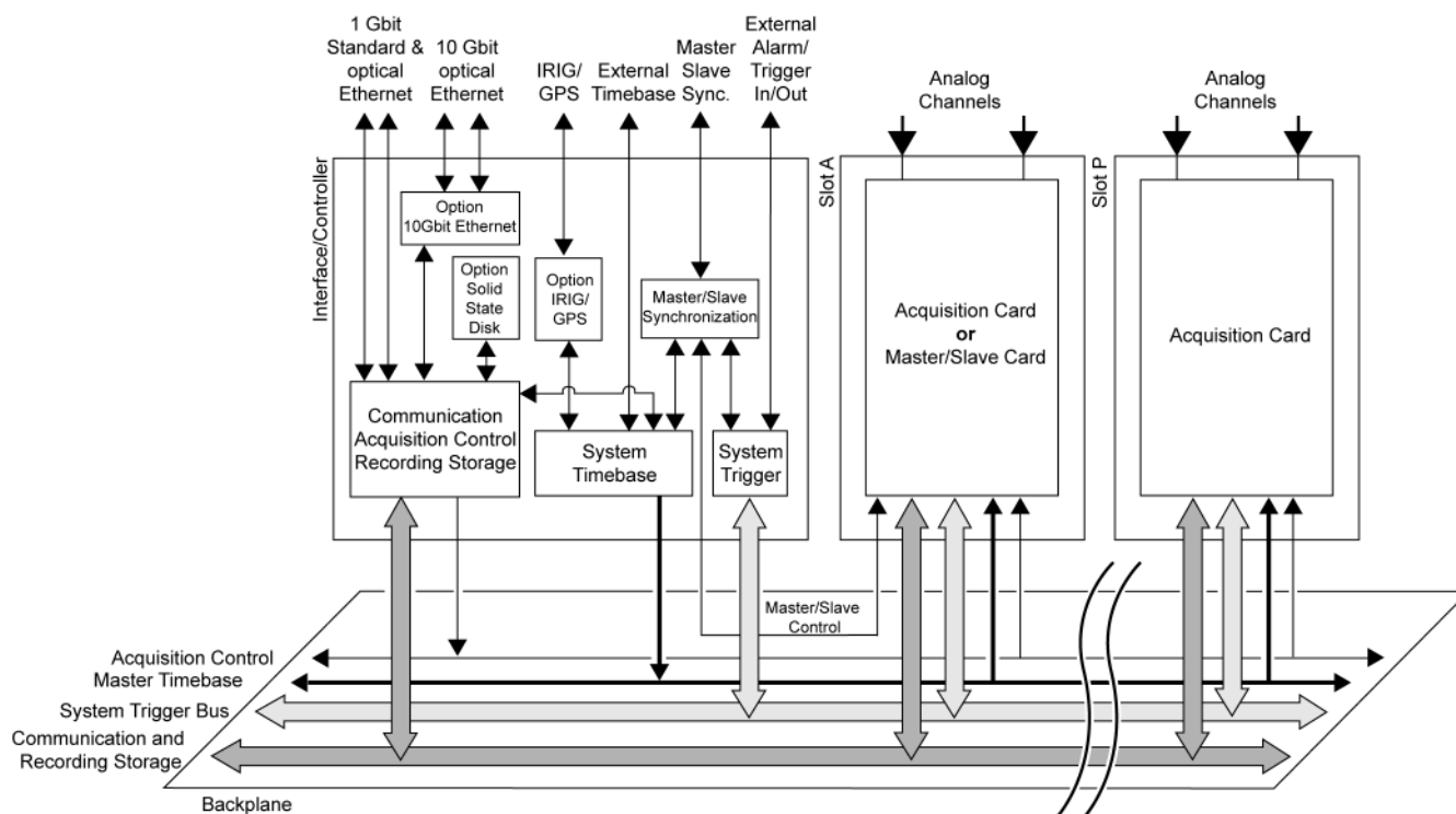
Figure 1.1: Block Diagram GEN16t Mainframe
